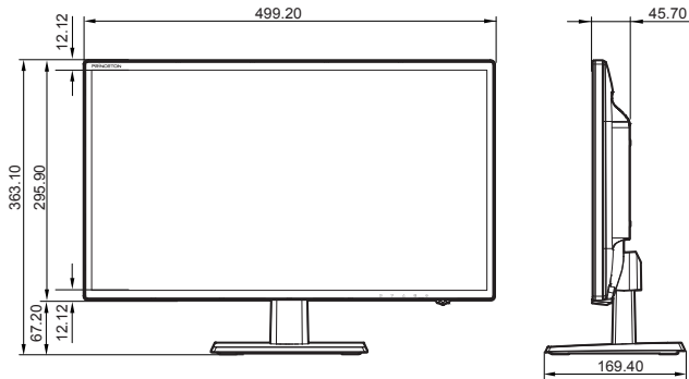
PTFBLT-22W / PTFWLT-22W 寸法図
