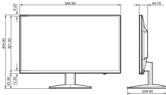
PTFBLT-22W / PTFWLT-22W 寸法図
